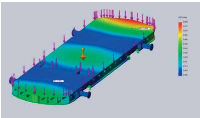
All sandwich plates are tested and optimized for capacity and rigidity according to FEM analysis
